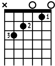
C MAJOR
