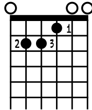
E MAJOR
