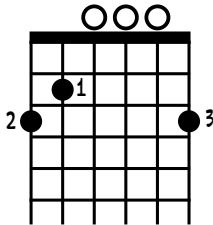
G MAJOR
