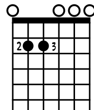
E MINOR
