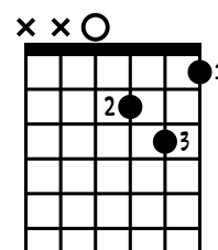
D MINOR
