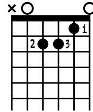
A MINOR
